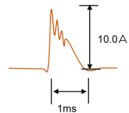
Fig. A : Inrush current waveform
