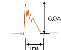
Fig. A : Inrush current waveform
