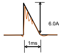
Fig. C : Inrush current waveform
