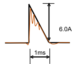
Fig. C : Inrush current waveform
