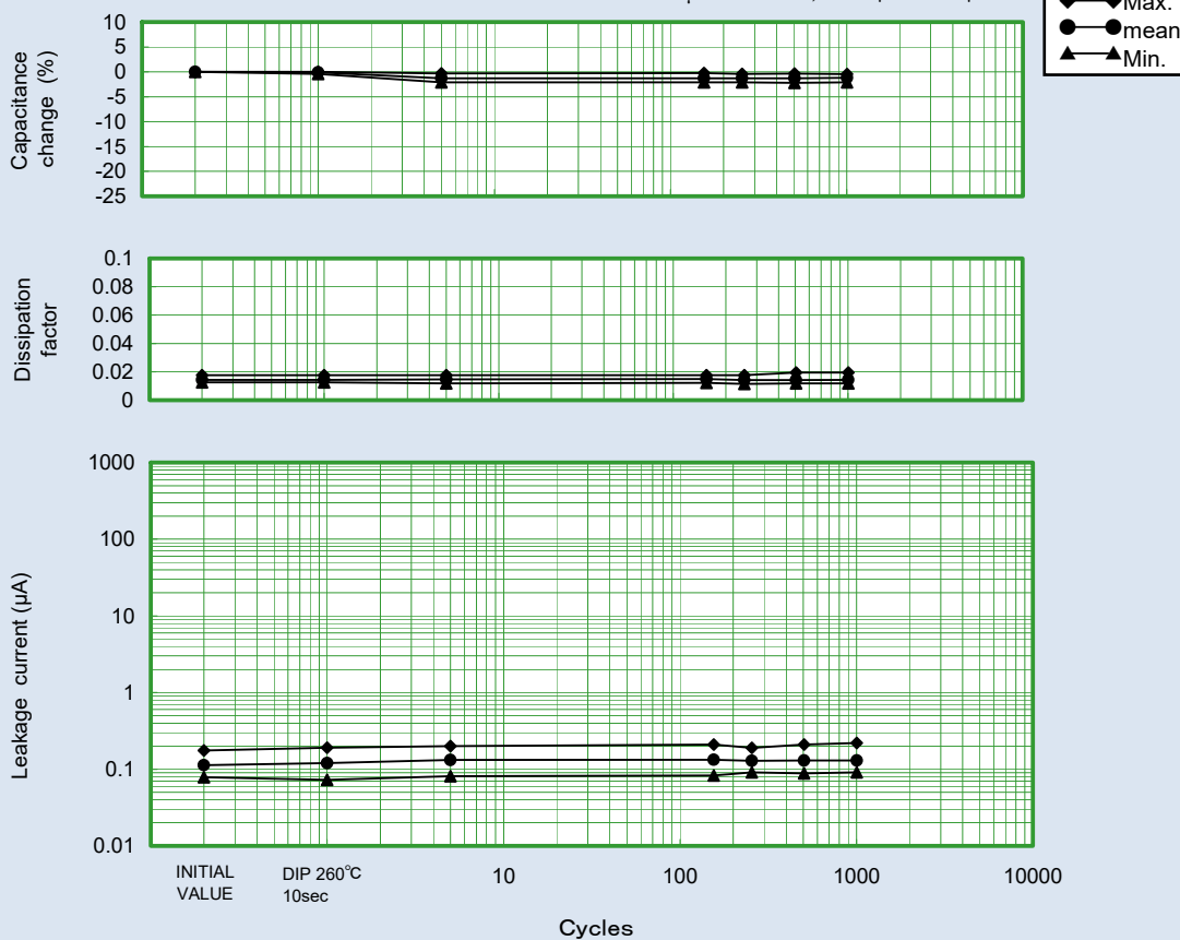
279M 35VDC-15 \mu F H-Case, Sample : 50pcs
